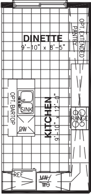
OPTIONAL KITCHEN #3
