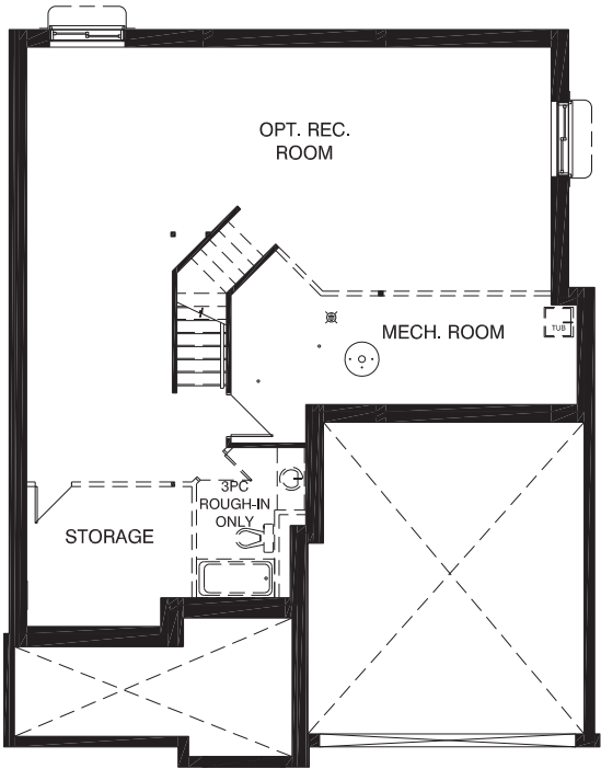
BASEMENT FLOOR - ELEVATION A
