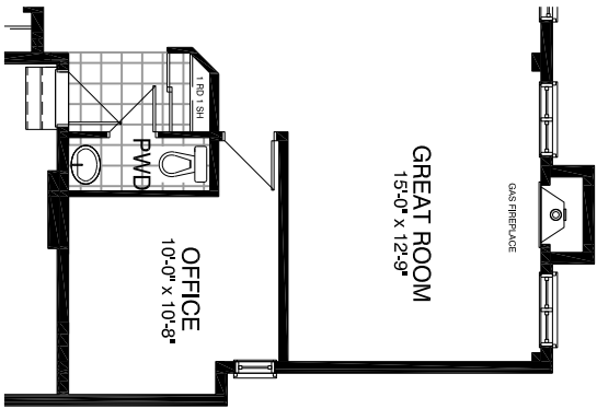
Ground Floor - Optional Office
