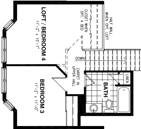
Second Floor - Loft Option
