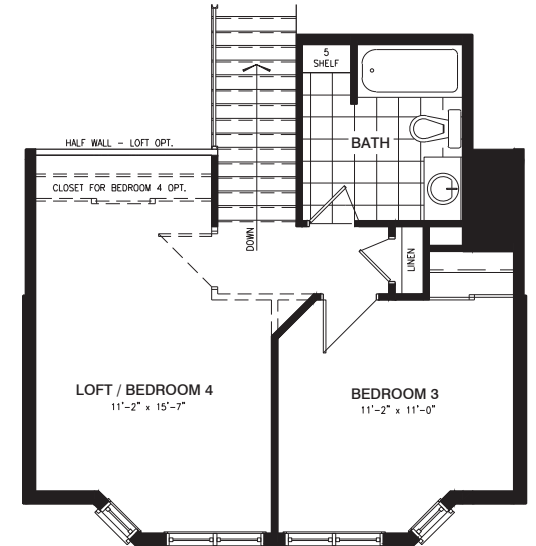
SECOND FLOOR - ELEVATION LOFT
