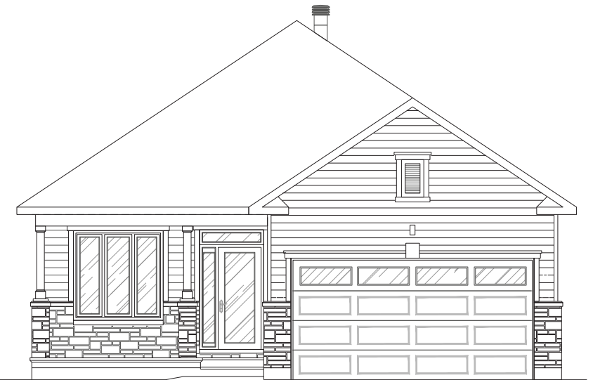
ELEVATION C
