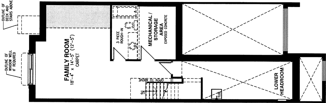
BASEMENT FLOOR
