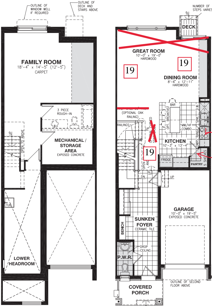
BASEMENT FLOOR
