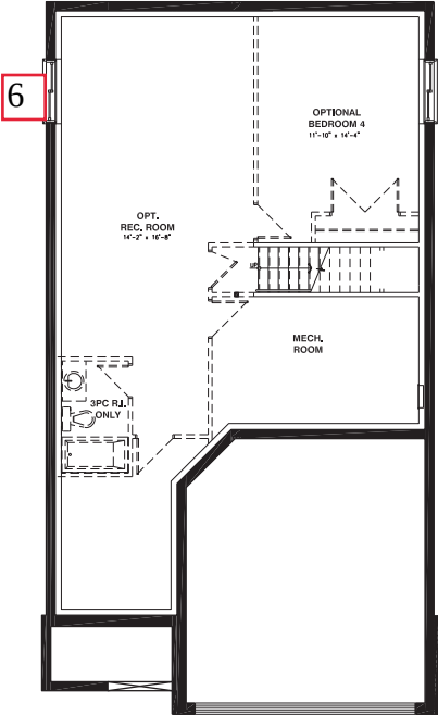
BASEMENT FLOOR
