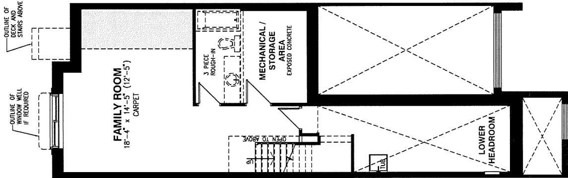
BASEMENT FLOOR
