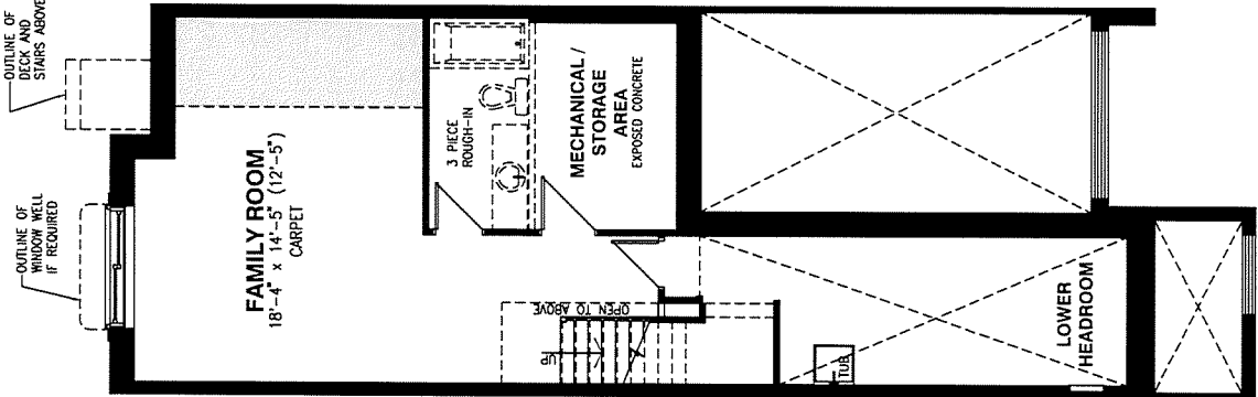
BASEMENT FLOOR
