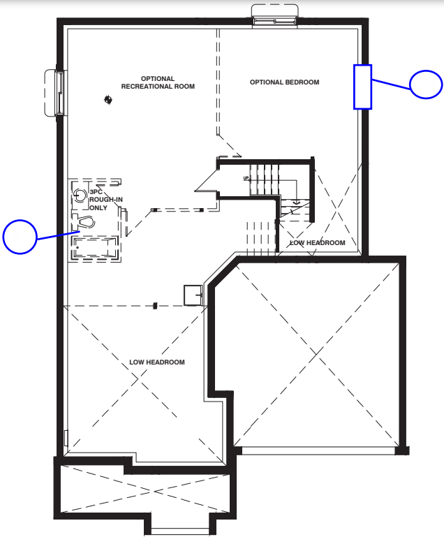
BASEMENT FLOOR - ELEVATION A
