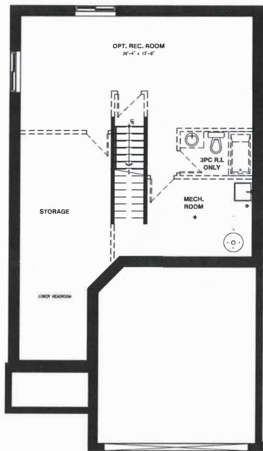
BASEMENT FLOOR
