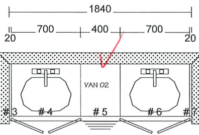
OPT. 4PC ENSUITE (DBL SINK) 2ND FLOOR
