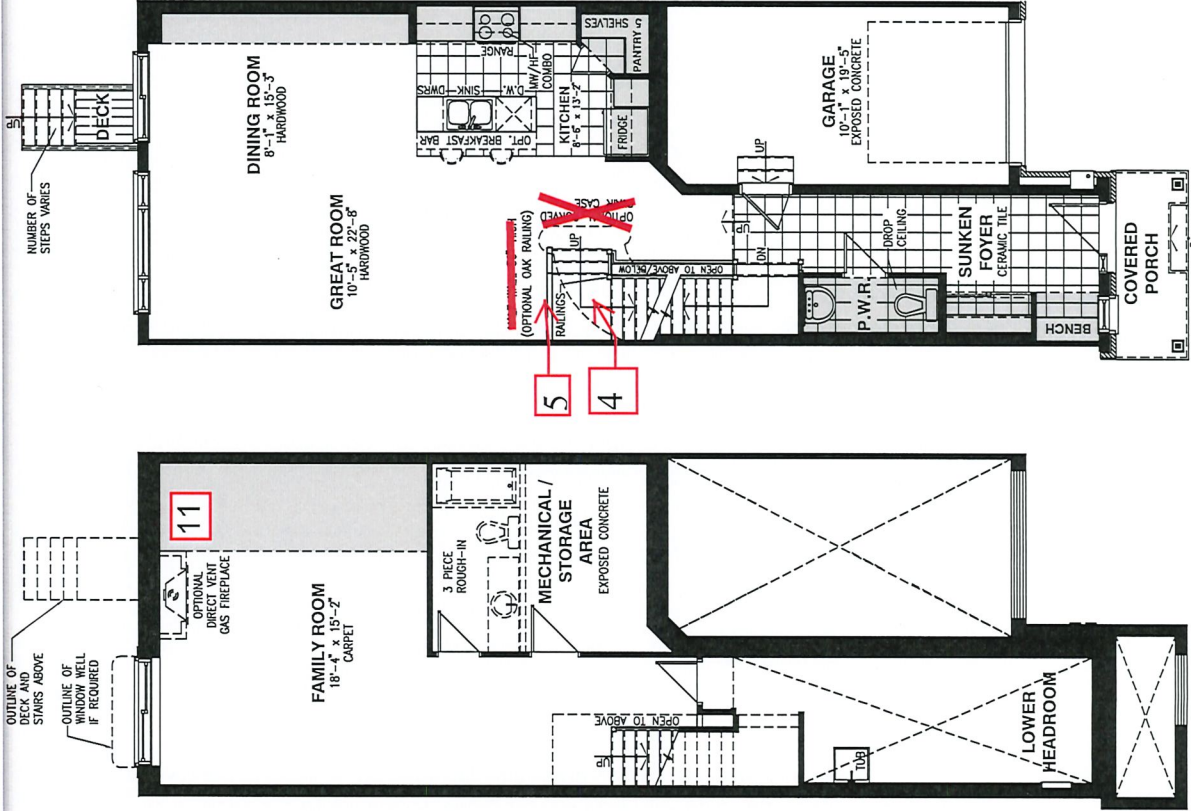
BASEMENT FLOOR
