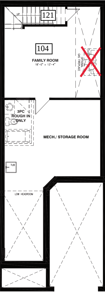
BASEMENT FLOOR
