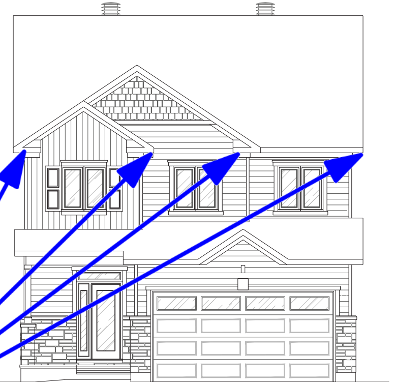
ELEVATION C
