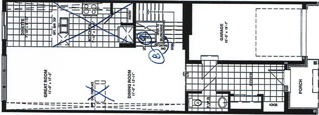
GROUND FLOOR
