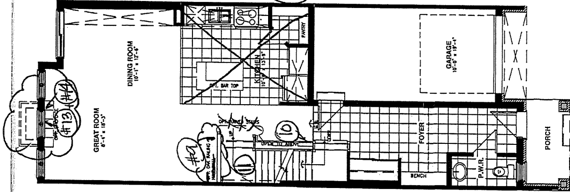
GROUND FLOOR
