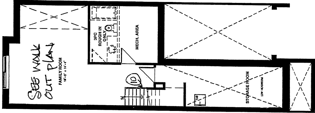
BASEMENT FLOOR
