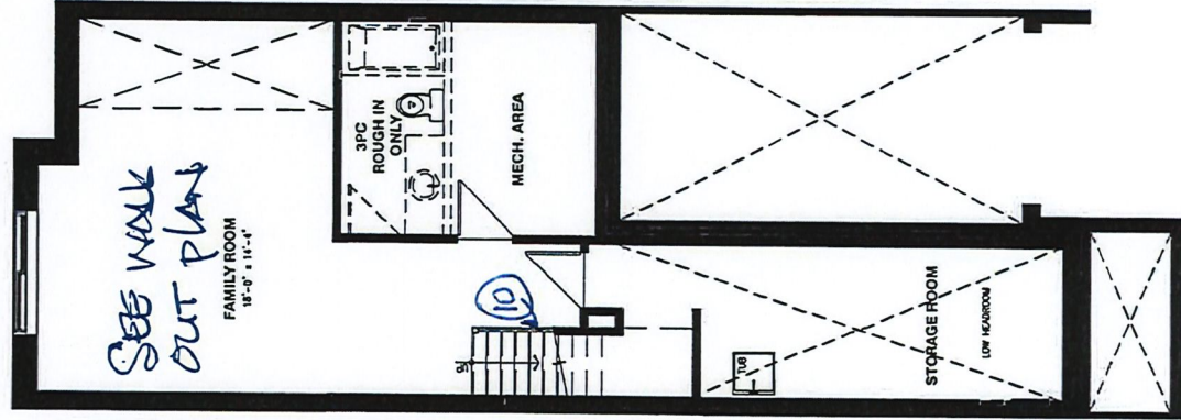
BASEMENT FLOOR
