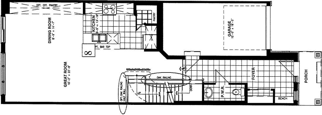
GROUND FLOOR
