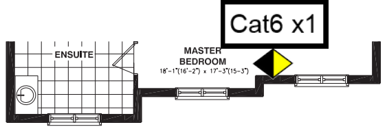
SECOND FLOOR - 3 & 4 BEDROOMS - ELEVATION C
