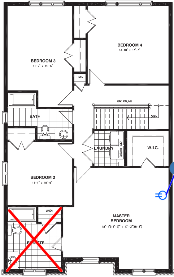
SECOND FLOOR - 4 BEDROOMS - ELEVATION A
