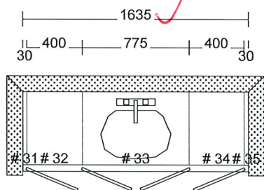
MAIN BATH
