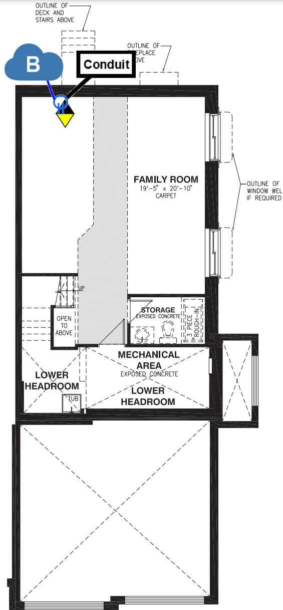
BASEMENT FLOOR
