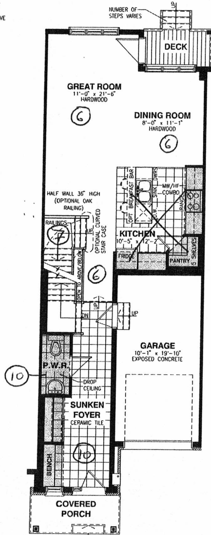
GROUND FLOOR
