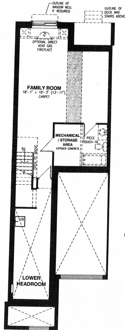
BASEMENT FLOOR
