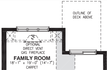
WALKOUT BASEMENT WHERE APPLICABLE
