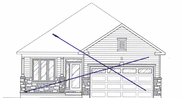
ELEVATION C
