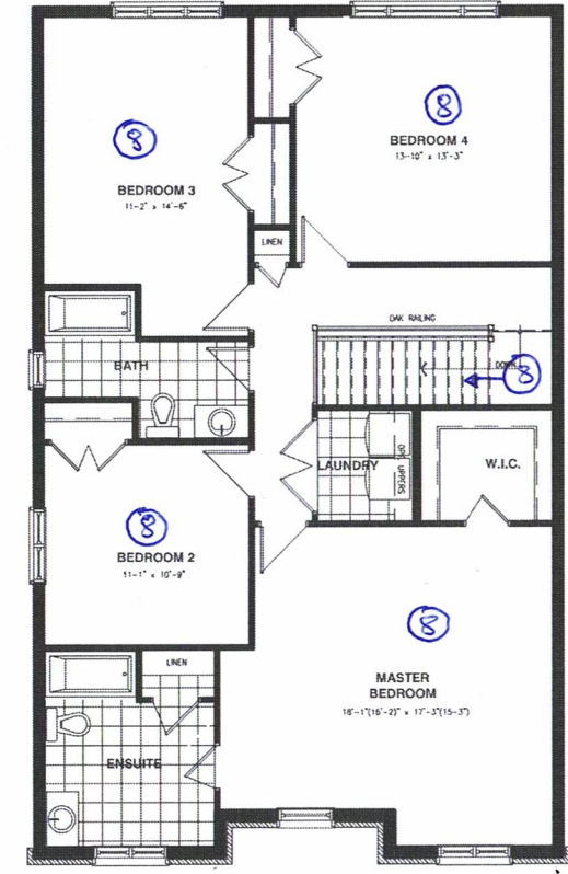
SECOND FLOOR - 4 BEDROOMS - ELEVATION C
