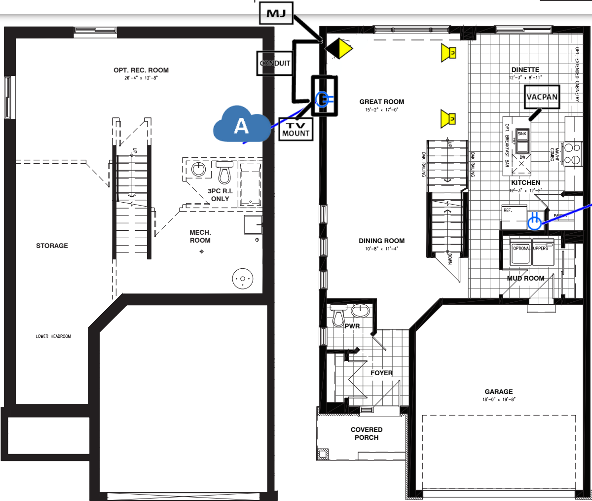
BASEMENT FLOOR
