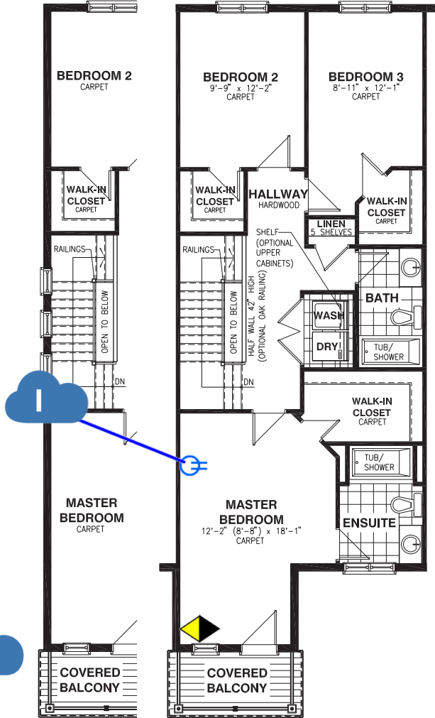
END UNIT SECOND SECOND FLOOR
