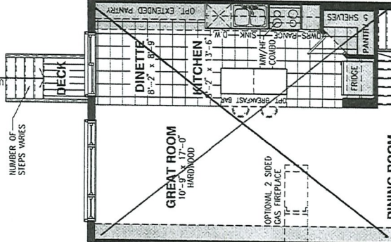
OPTIONAL KITCHEN #2
