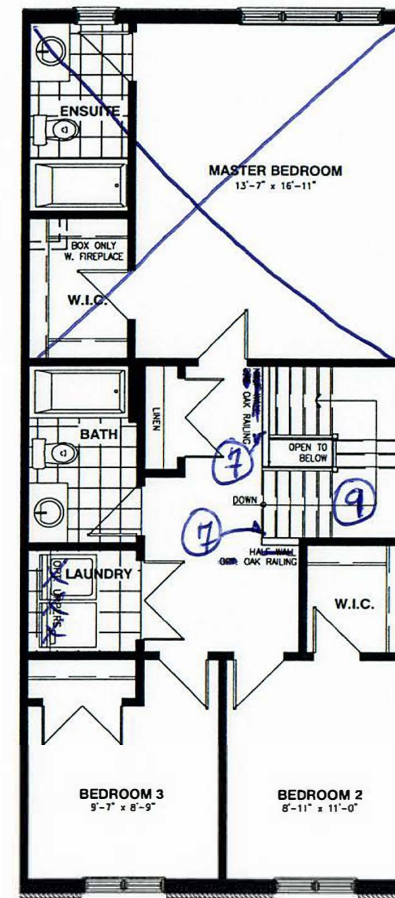
SECOND FLOOR
