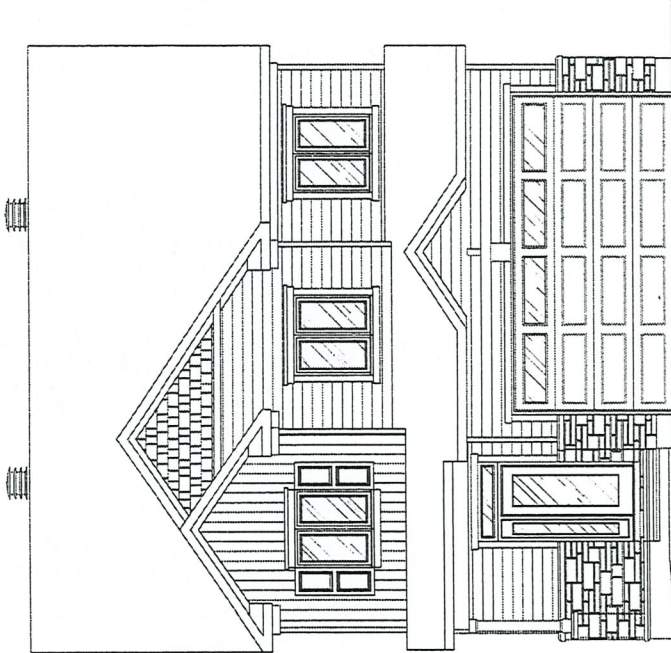
ELEVATION C
