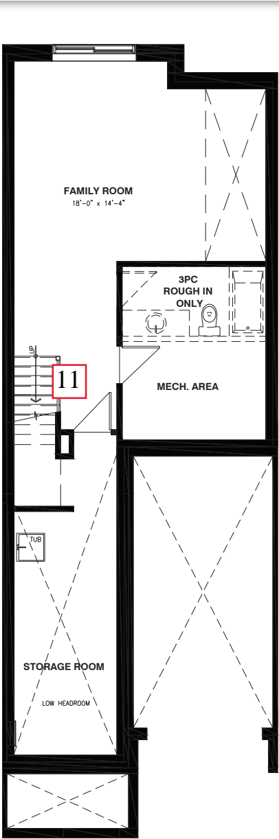
BASEMENT FLOOR
