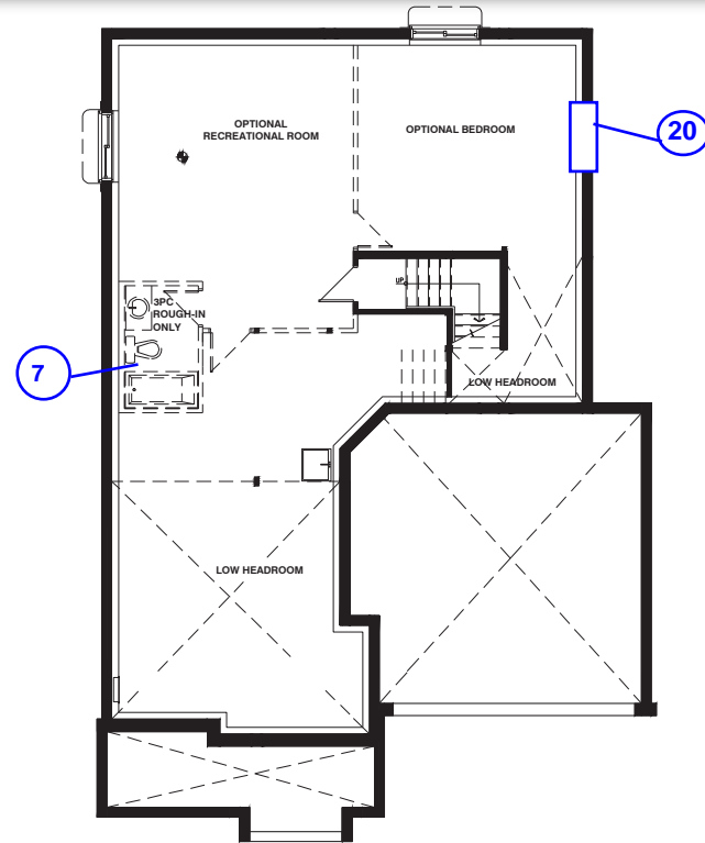
BASEMENT FLOOR - ELEVATION A
