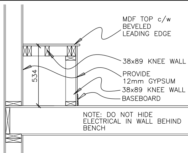
5a. CLOSED (STANDARD) WINDOW SEAT DETAILS
