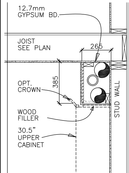
3a. DCBH (STANDARD) BULKHEAD DETAILS OVER CABINETS
