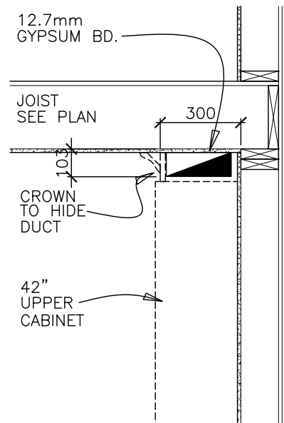
3a. DCBH (STANDARD) BULKHEAD DETAILS OVER CABINETS
