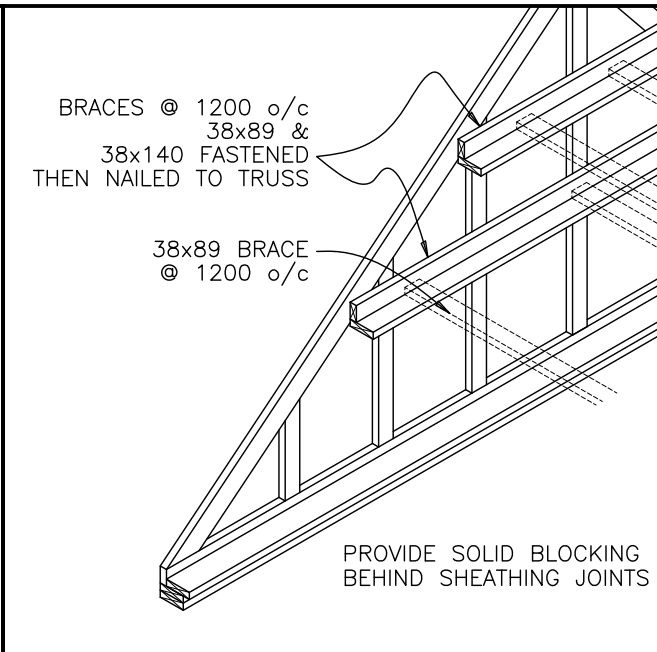
4. TYPICAL GABLE TRUSS BRACING DETAIL
