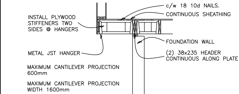
2. SECTION THROUGH (CANTILEVER FIREPLACE DETAIL) CANTILEVERED FIREPLACE DETAIL
