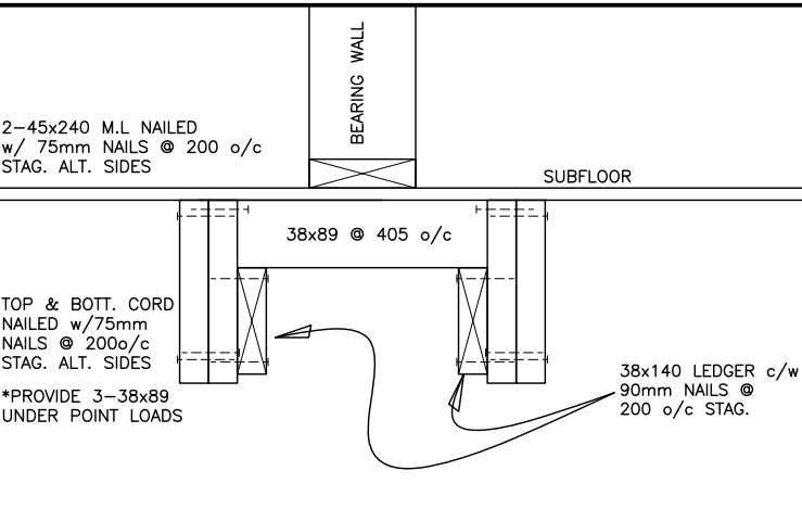
7a. SECTION THROUGH LOAD BEARING WALL PARALLEL TO JST. LVL BEAMS LOAD BEARING MECHANICAL WALL SUPPORT
