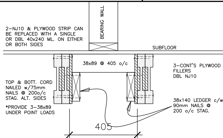
7b. SECTION THROUGH LOAD BEARING WALL PARALLEL TO JST. NJ10 BEAMS
