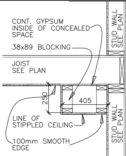
6b.TYPICAL COFFERED CEILING
