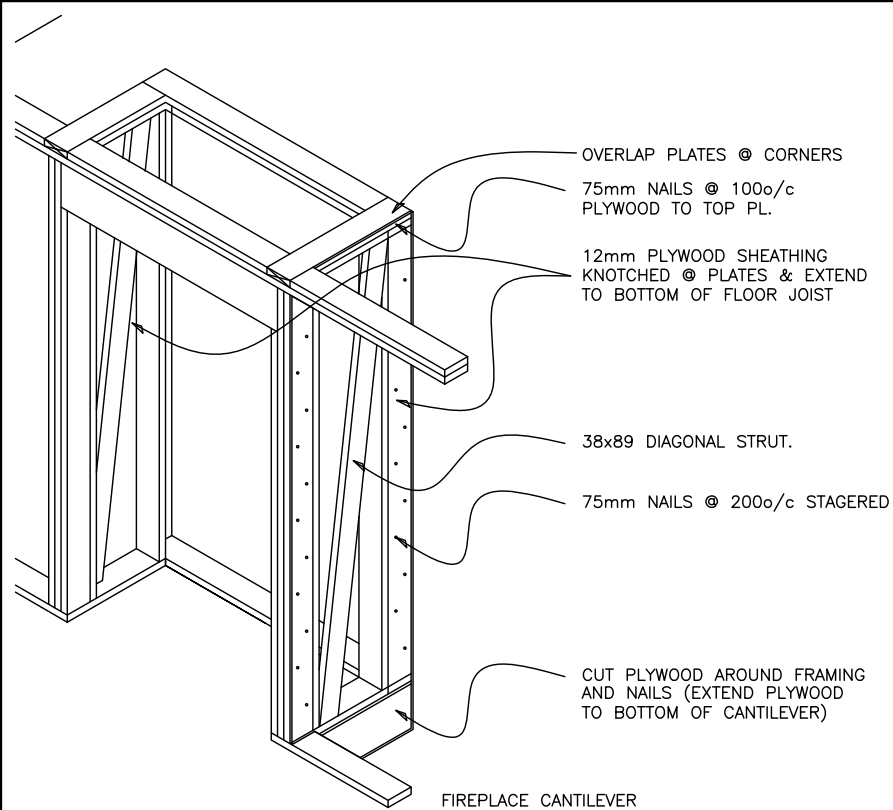
1. ISO (CANTILEVER FIREPLACE DETAIL)
