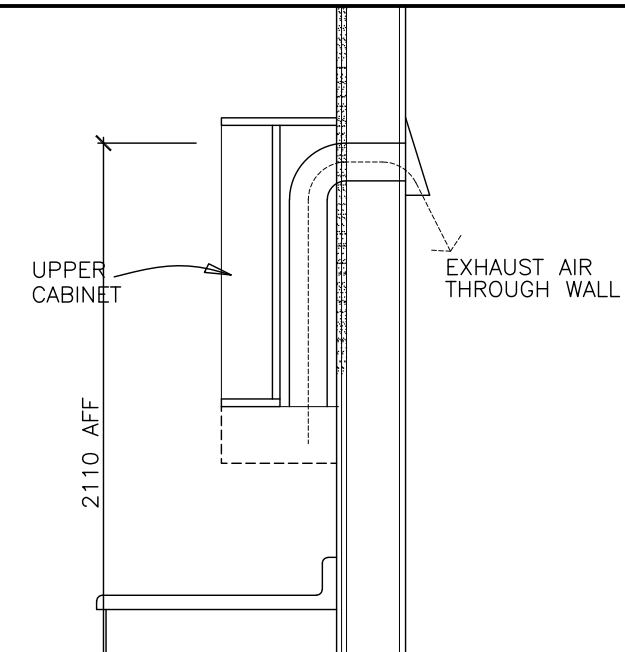
3d. STANDARD RANGE EXHAUST THROUGH REAR CABINET
