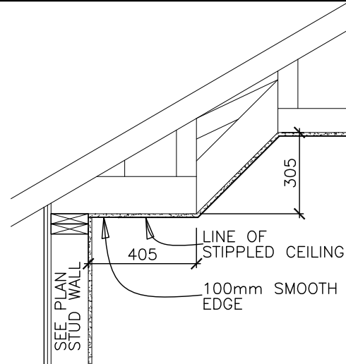
6a.TYPICAL COVE CEILING INTO TRUSSES COFFER AND COVE CEILING DETAILS
