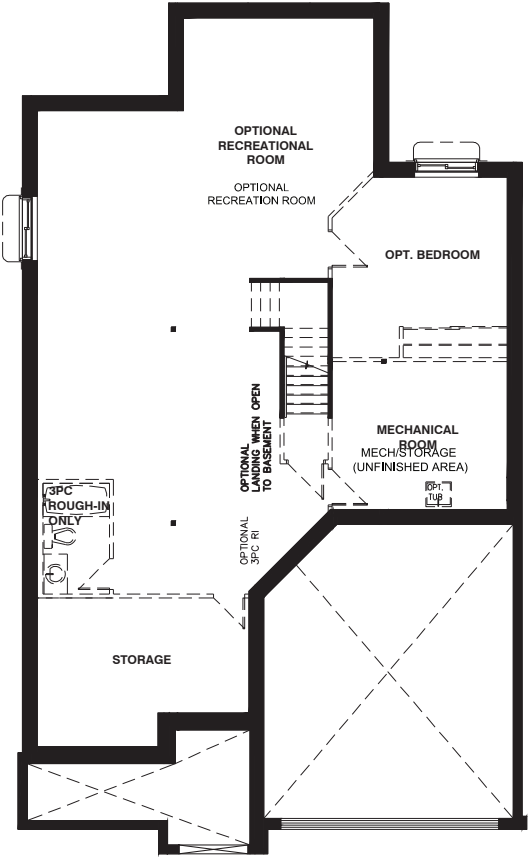
BASEMENT FLOOR - ELEVATION A & B C
