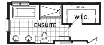
5PC ENSUITE UPGRADE
