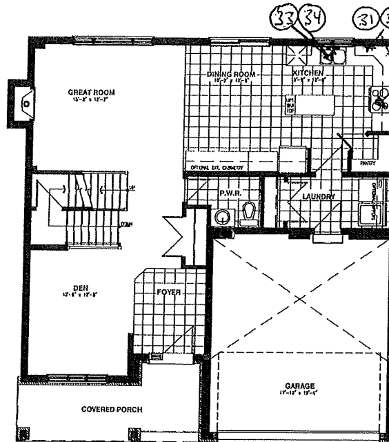
GROUND FLOOR - ELEVATION A & B
