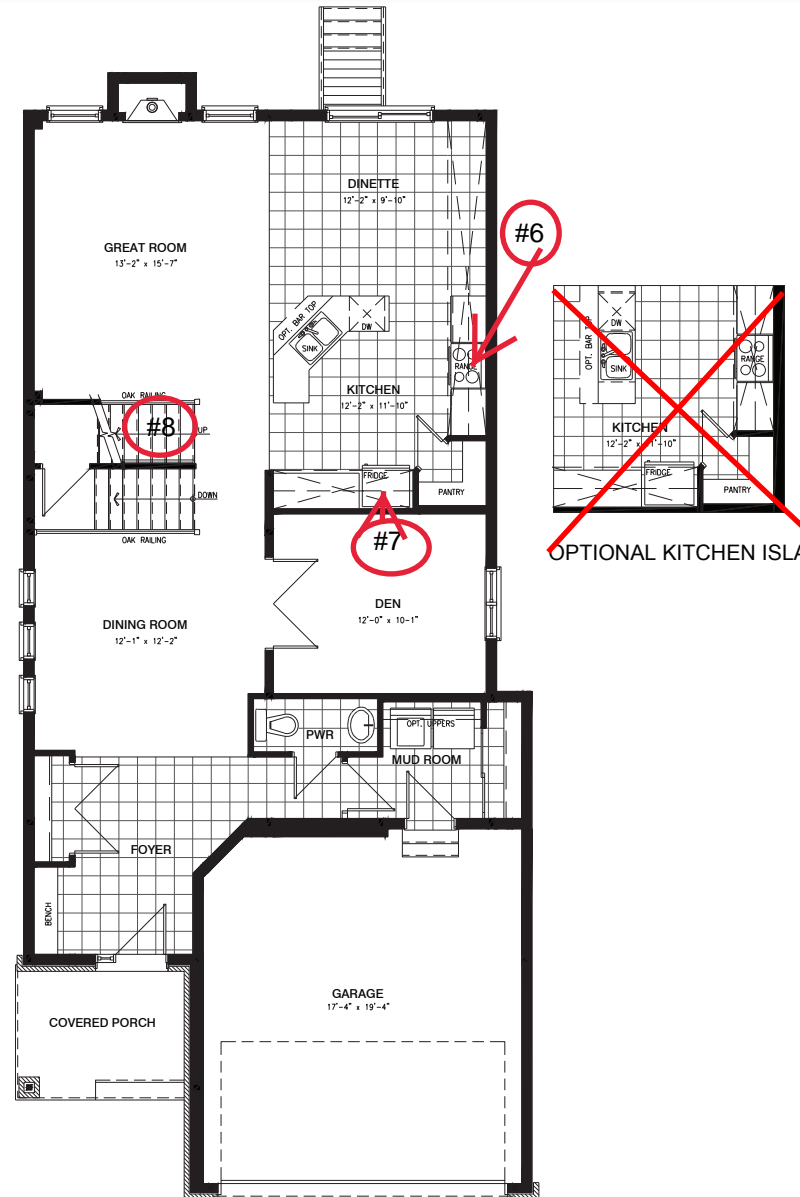
GROUND FLOOR
