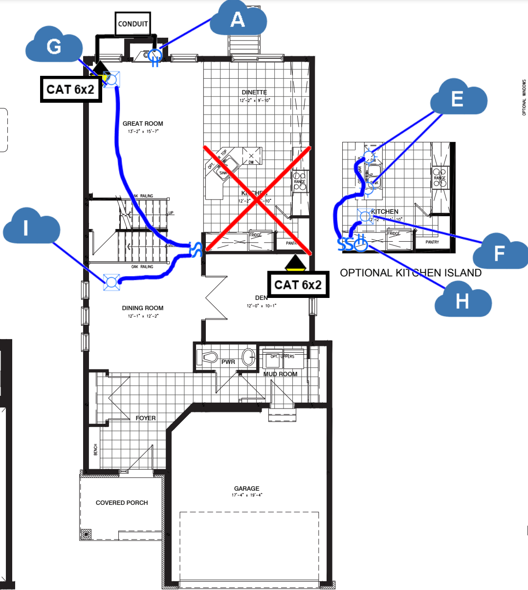
GROUND FLOOR
