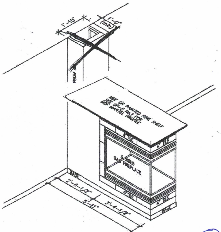
UPG. OPT. 3-WAY FIREPLACE W/ SHELF
