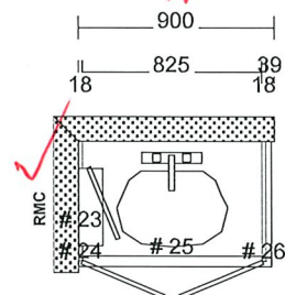
MAIN BATH 2ND FLOOR
