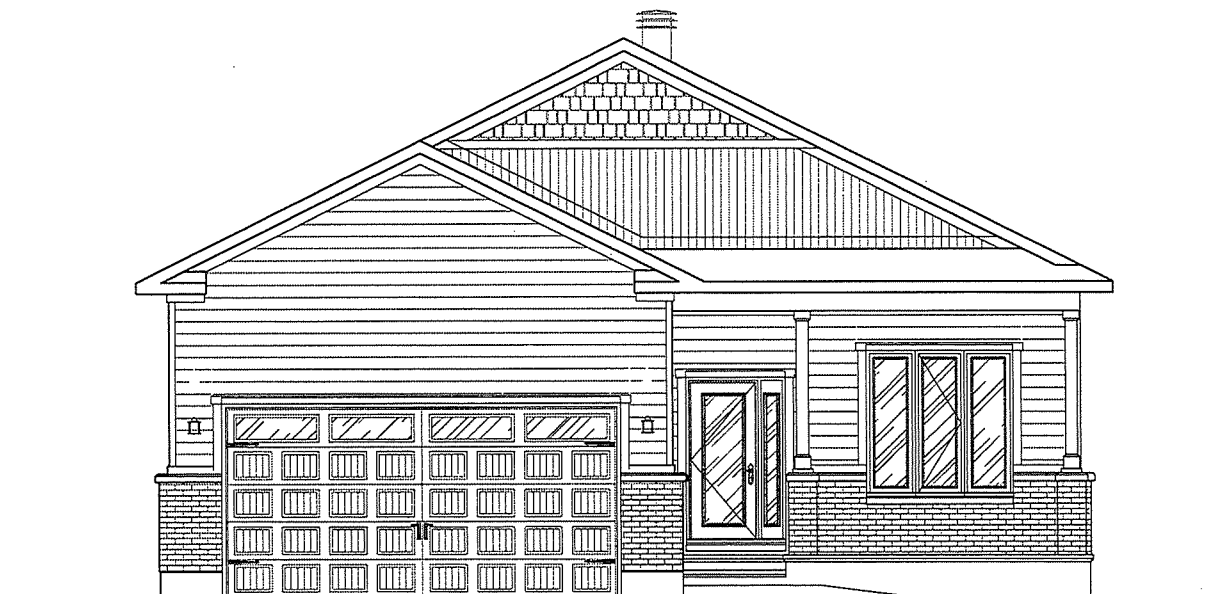
FRONT ELEVATION
