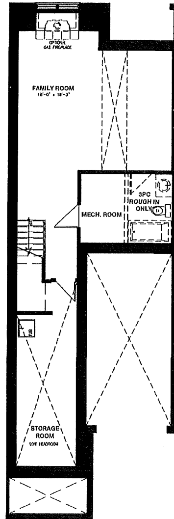
BASEMENT FLOOR
