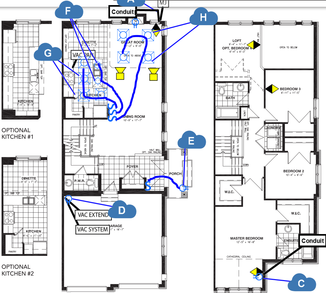
GROUND FLOOR
