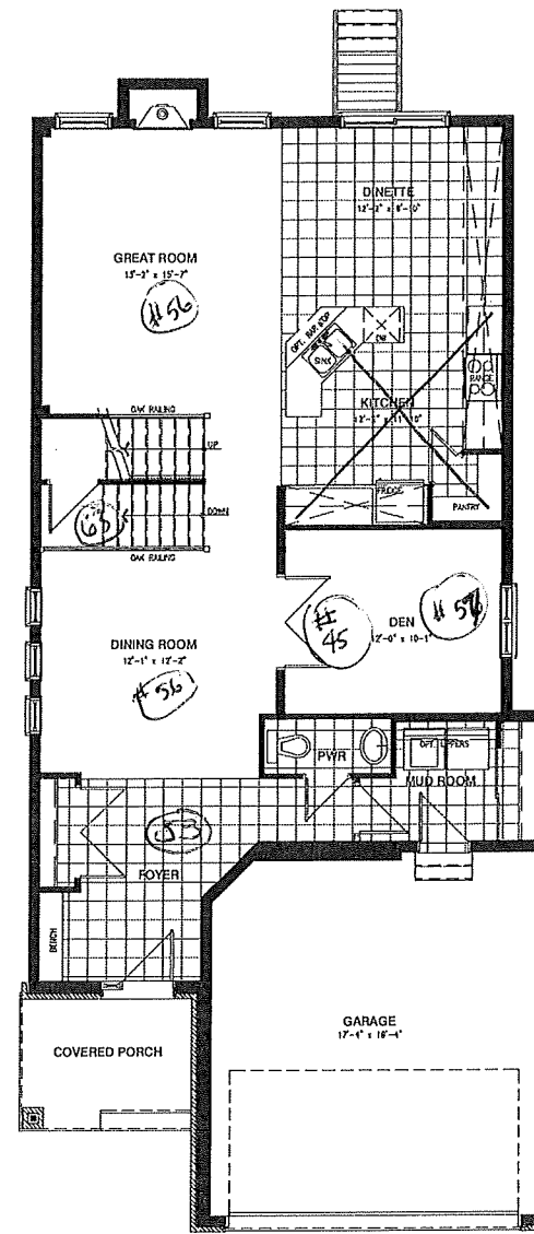
GROUND FLOOR
