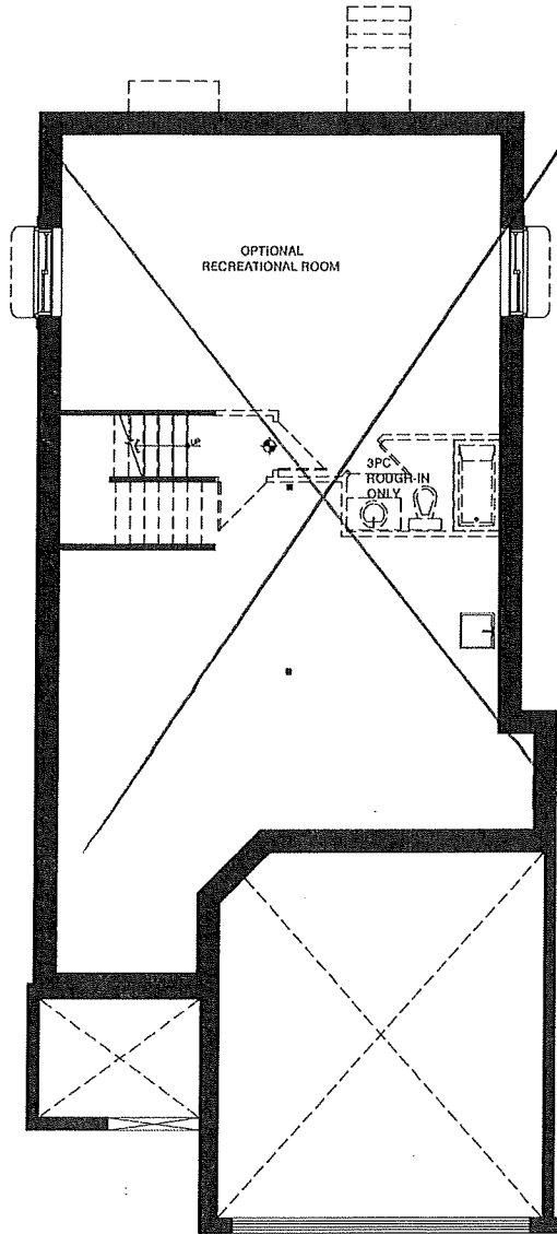
BASEMENT FLOOR
