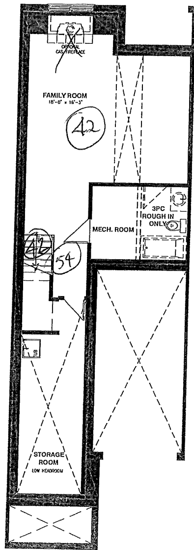
BASEMENT FLOOR
