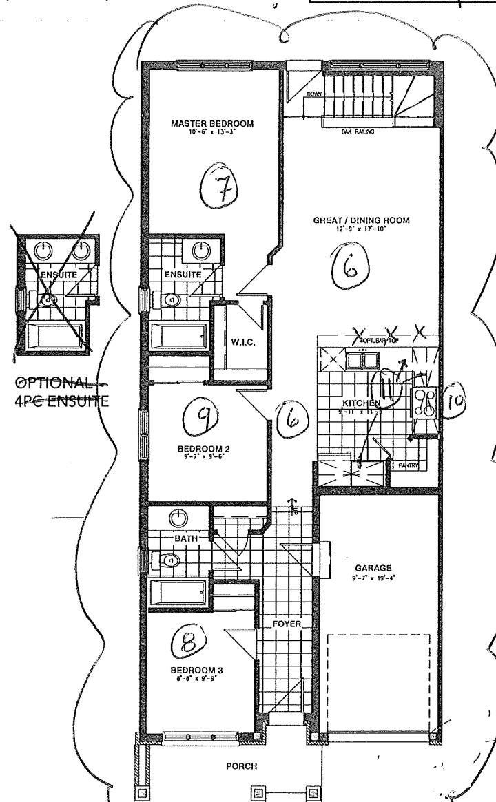
GROUND FLOOR STANDARD 3 BEDROOM PLAN
