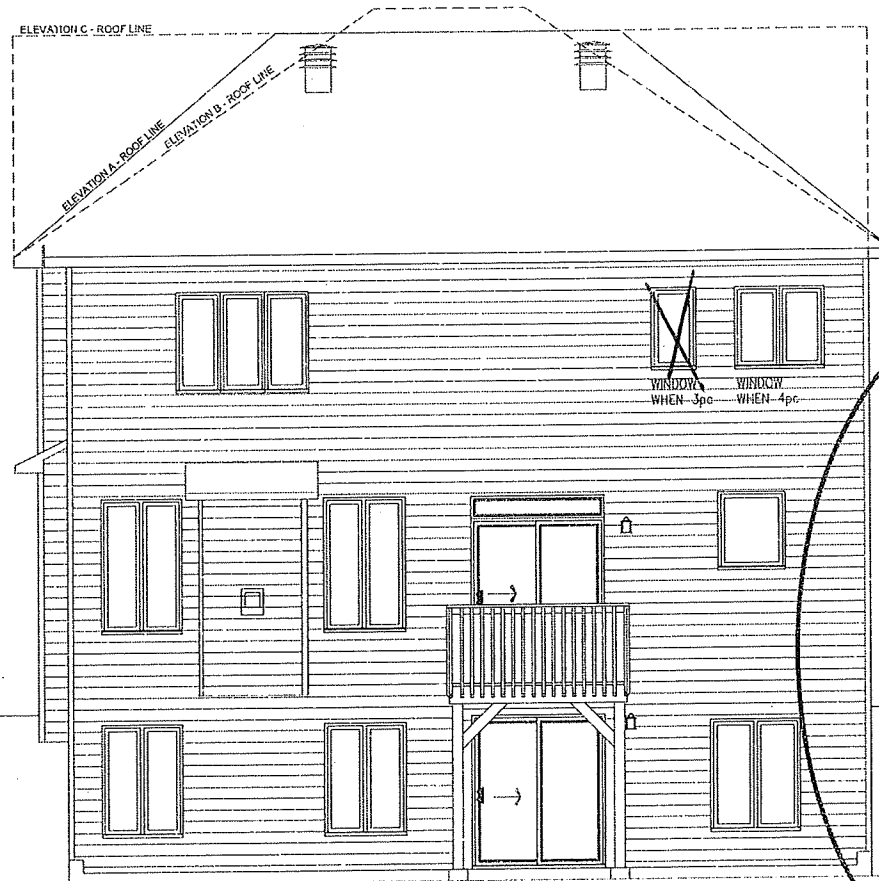
REAR ELEVATION - WALKOUT BASEMENT
