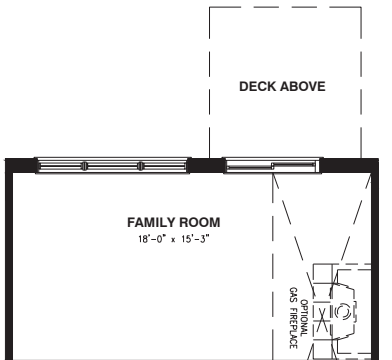
BASEMENT WALKOUT WHERE APPLICABLE
