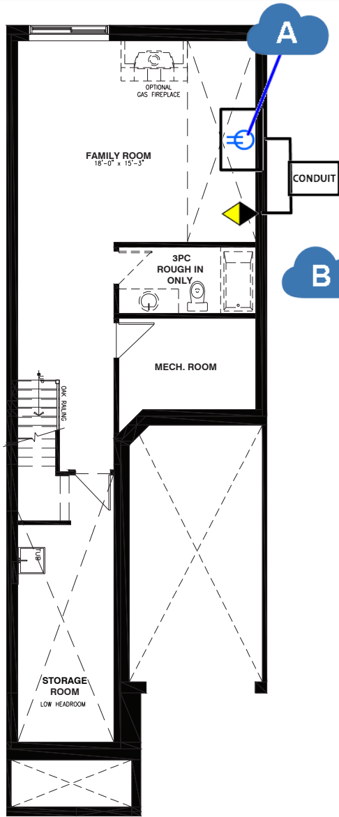
BASEMENT FLOOR
